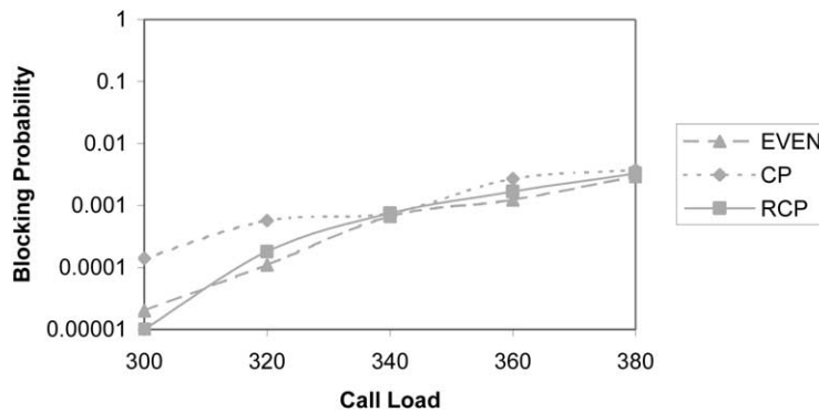
Fig. 14. Simulation results for configuration C of model 2, with resource-based routing.
