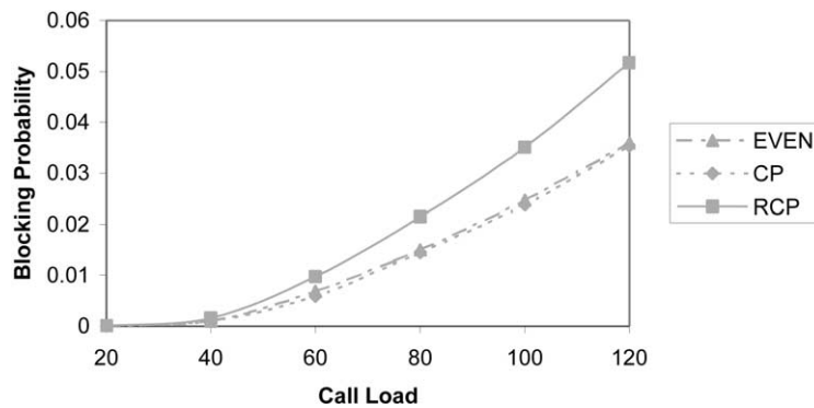
Fig. 11. Simulation results for configuration C of model 2.
