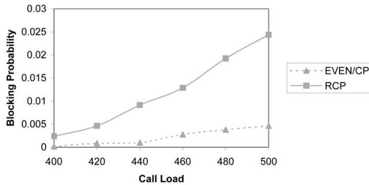
Fig. 9. Simulation results for configuration A of model 2.
