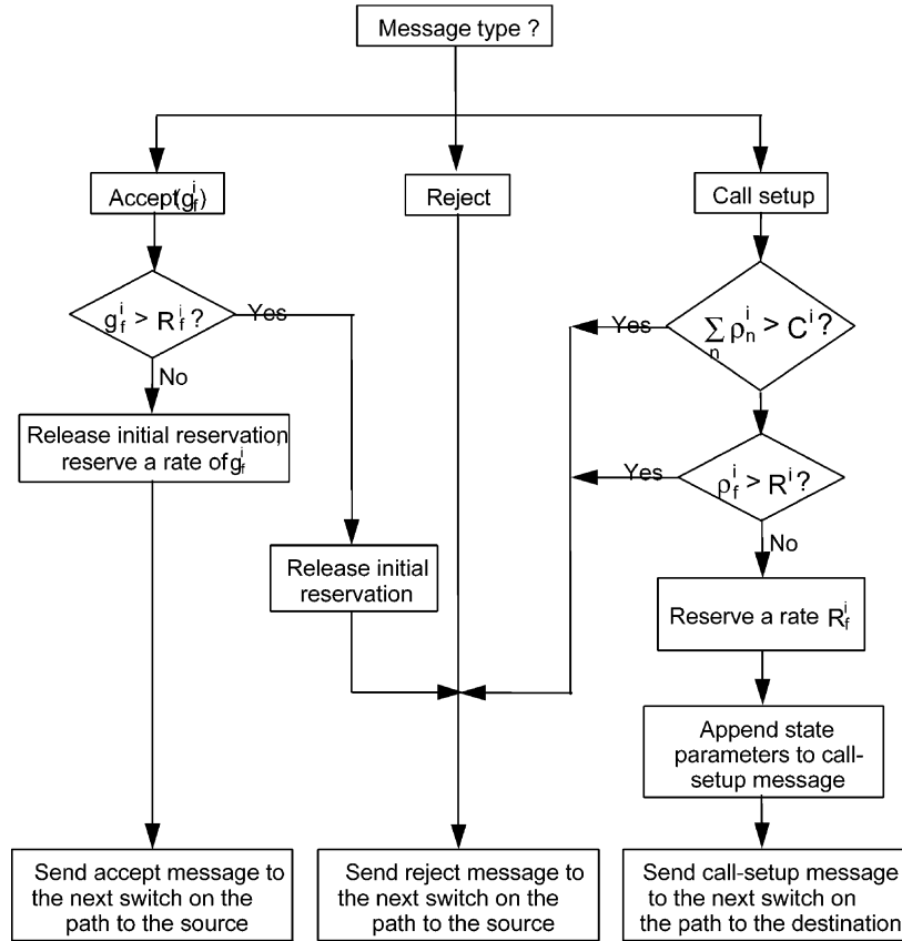
Fig. 1. Part (A) of the CAC algorithm with local stability imposed.
