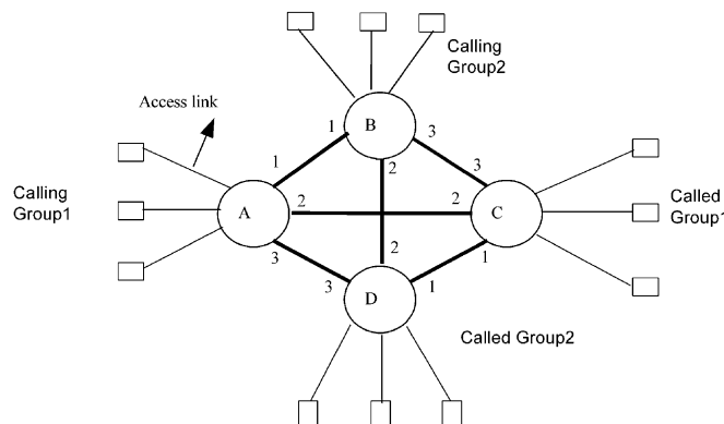
Fig. 7. Four node full-mesh network.
