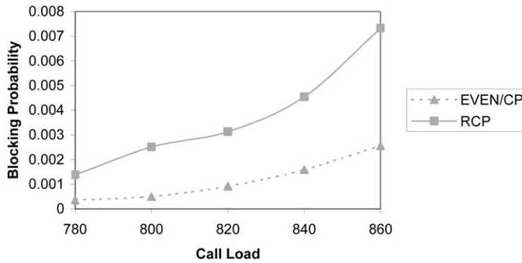
Fig. 12. Simulation results for configuration A of model 2, with resource-based routing.
