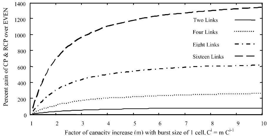
Fig. 5. Gain of CP/RCP over EVEN policy with link capacity increasing exponentially along the path.
