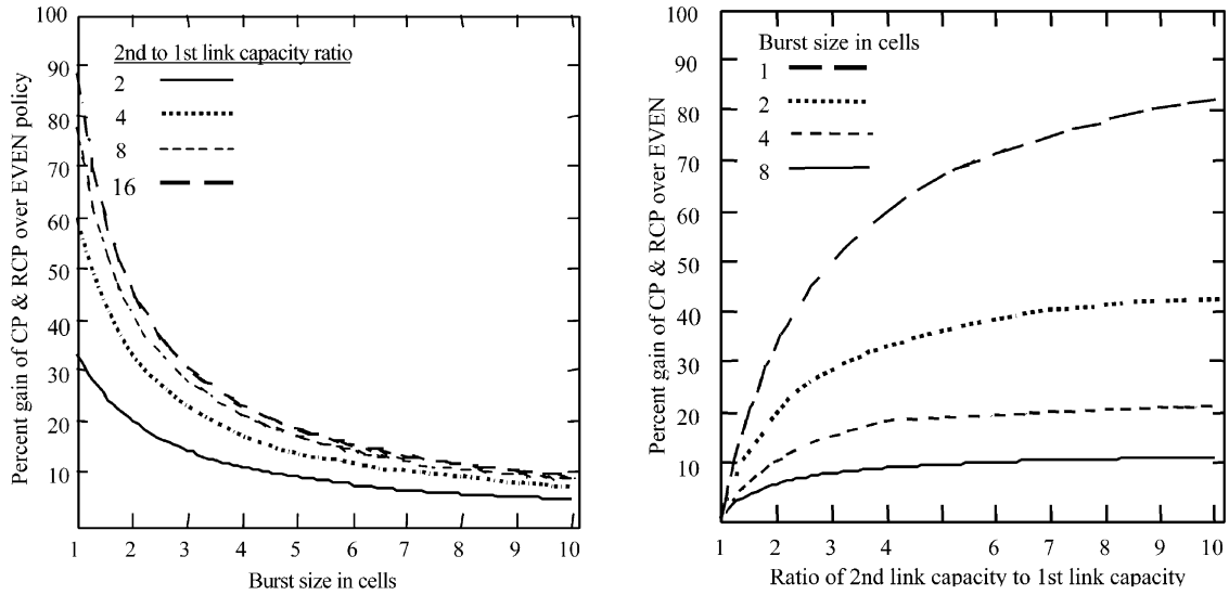
Fig. 4. Results for three switches (2 links).
