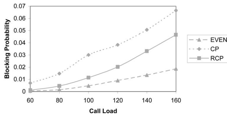
Fig. 10. Simulation results for configuration B of model 2.
