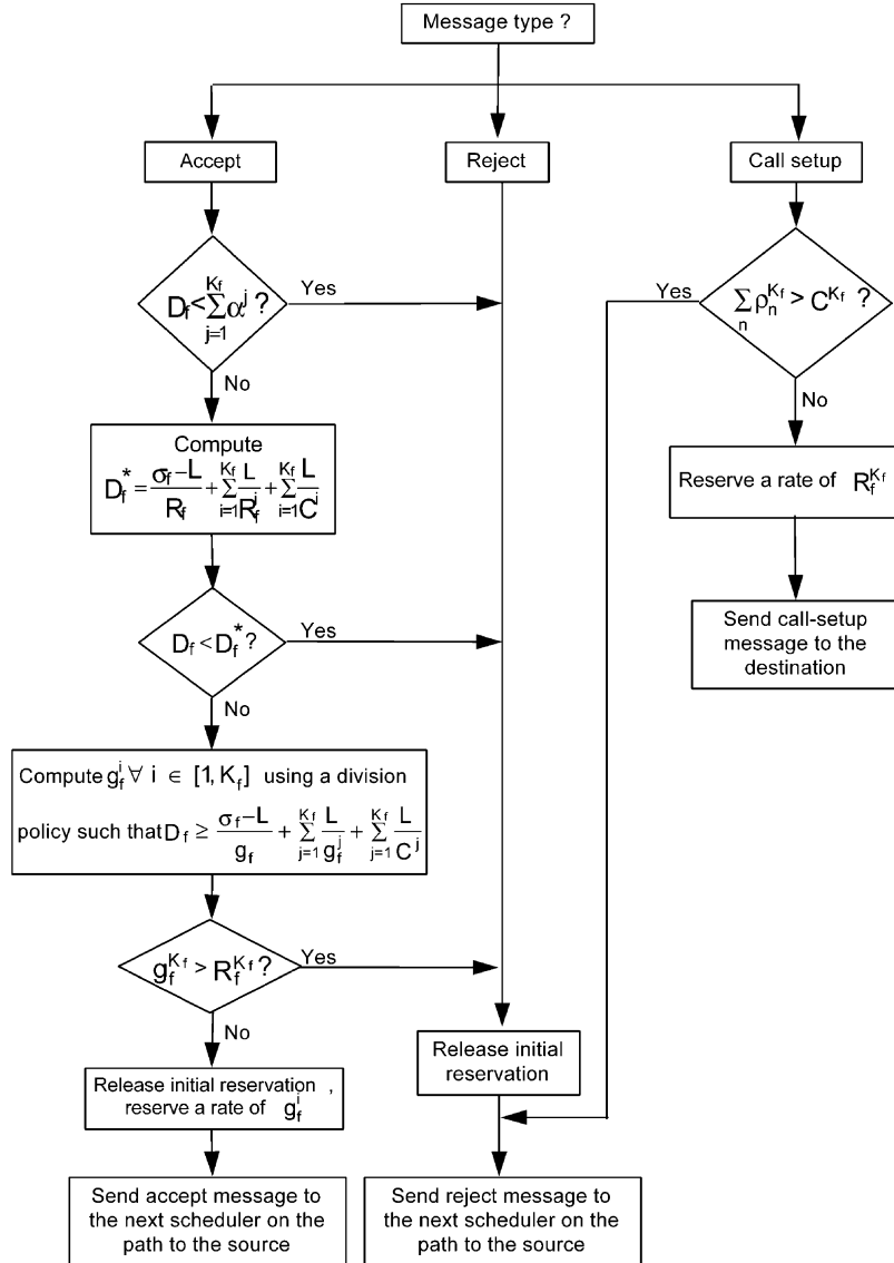
Fig. 2. Part (B) of the CAC algorithm used with local stability imposed.
